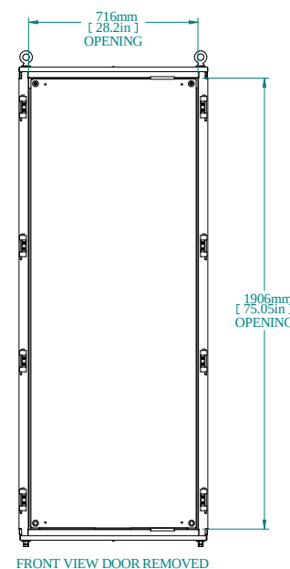
FRONT VIEW DOOR REMOVED
