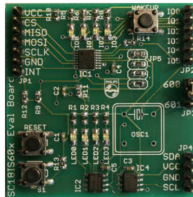
SPI to I 2 C Master
