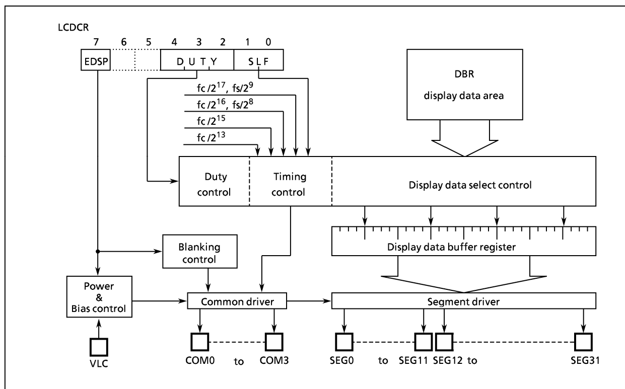
Figure 2-42. LCD driver
