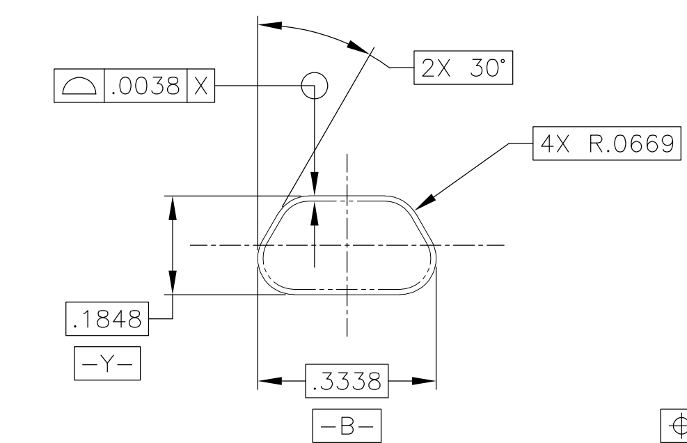
INTERFACE DETAIL
