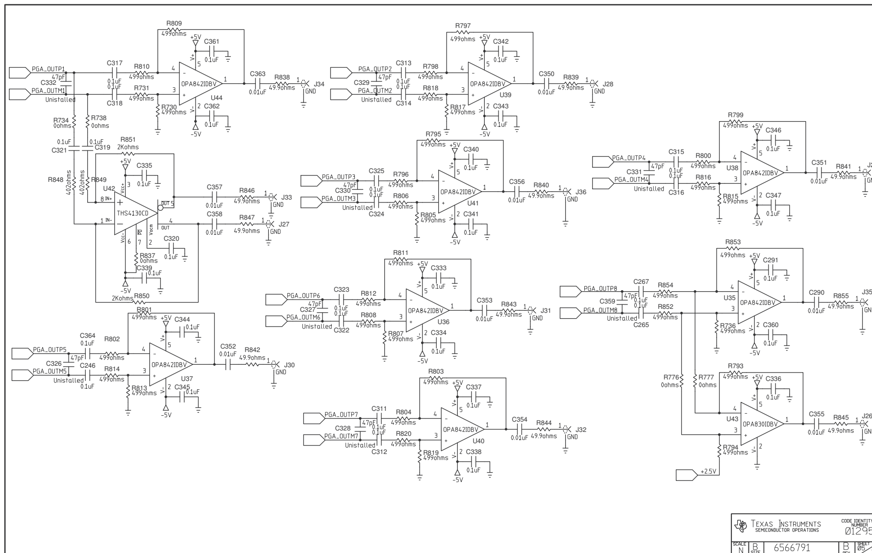
Figure 22. Schematic 5 of 10
