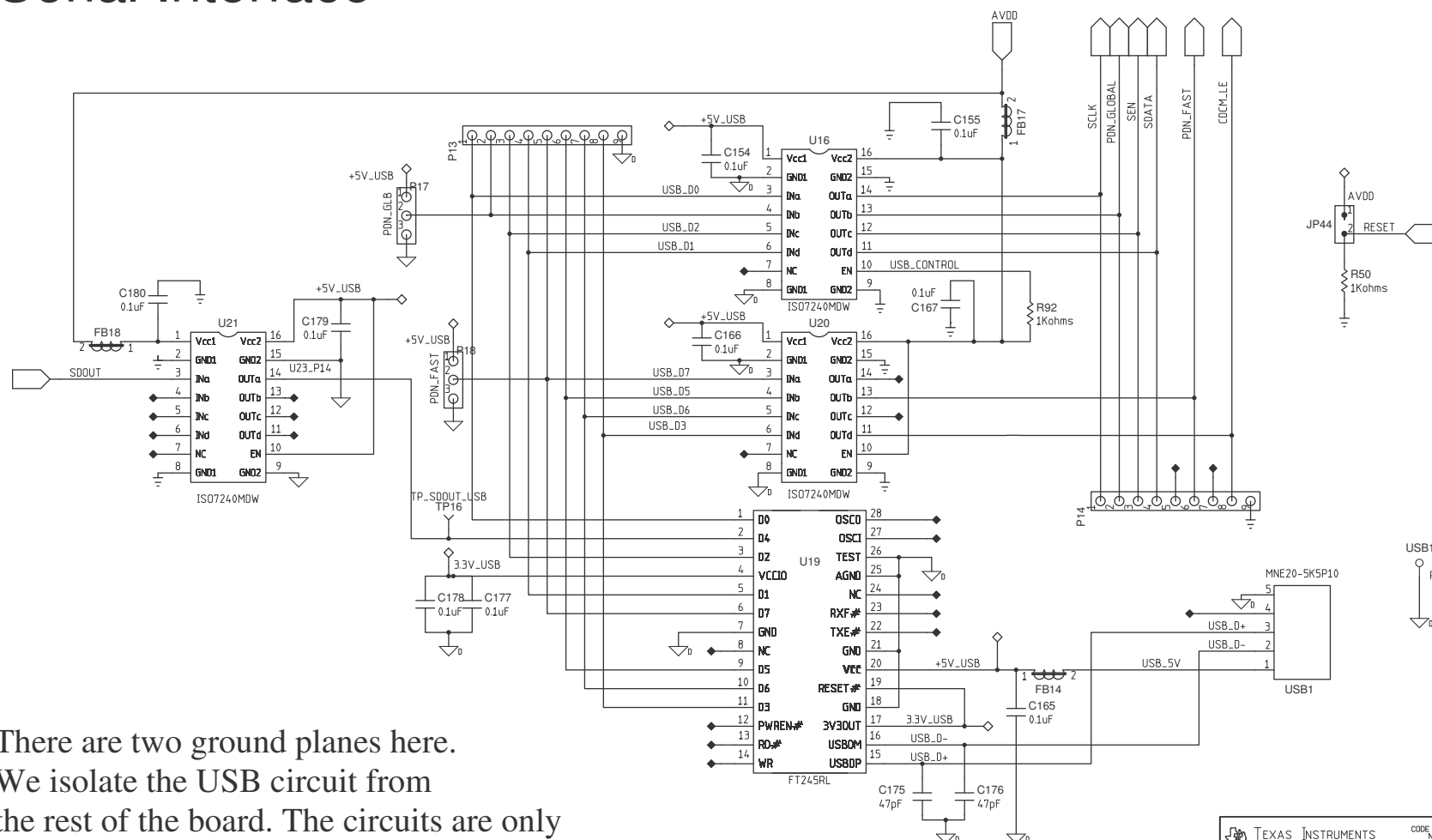
Figure 26. Schematic 9 of 10
