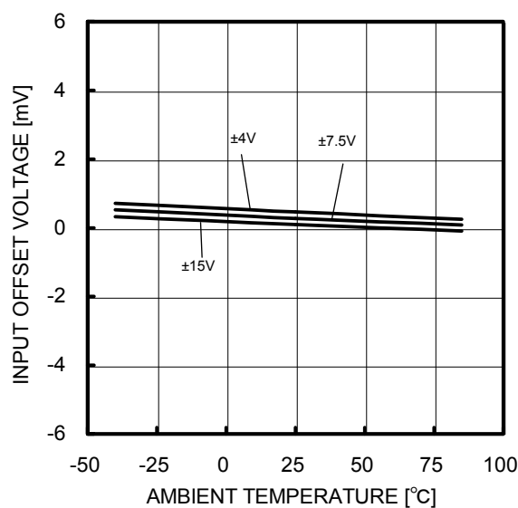
Figure 11. Input Offset Voltage - Ambient Temperature ( V_{ICM}=0V , V_{OUT}=0V )
