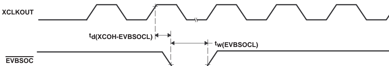
Figure 6–20. \overline{\text{EVBSOC}} Timing
