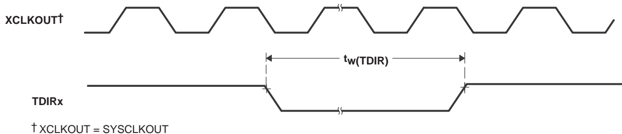
Figure 6–18. TDIRx Timing
