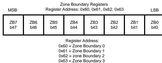
Figure 38. Zone Boundary Register Descriptions
