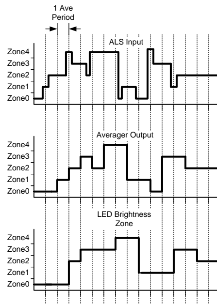
Figure 44. Ambient Light Input to Backlight Mapping
