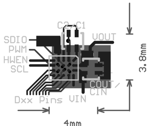
Figure 2. Minimum Layout
