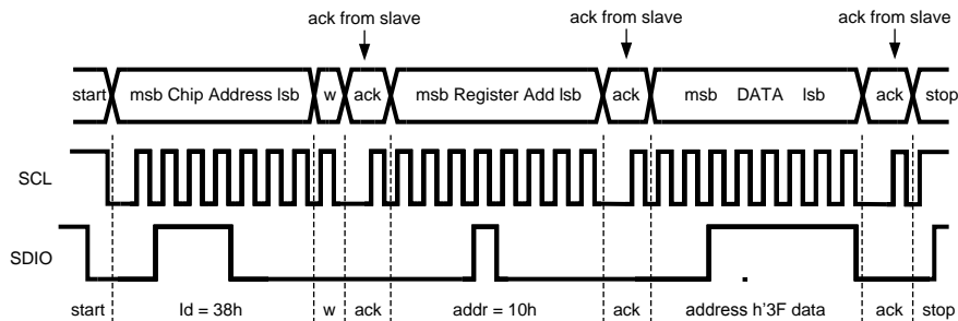
Figure 29. Write Cycle
