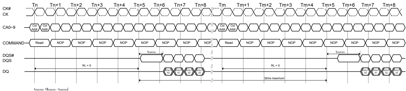
Figure 15. t_{DQSCKDL} timing
