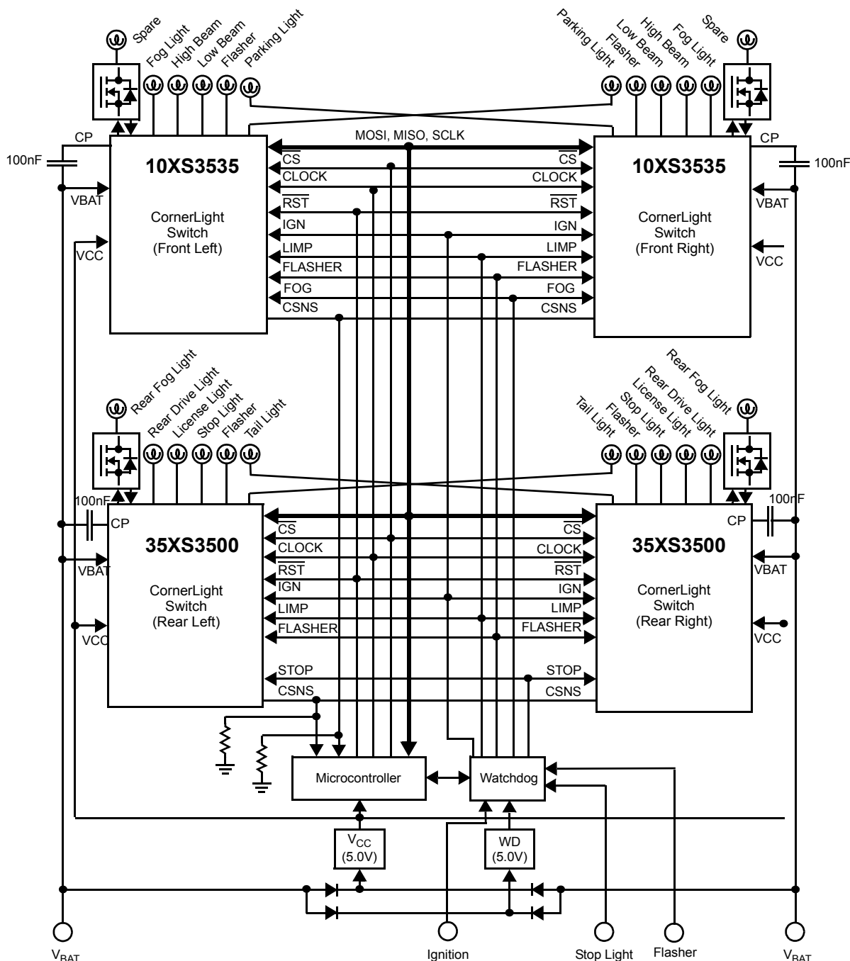
Figure 19. Typical Application
