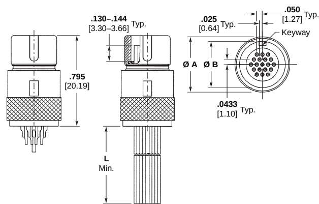
Plug (19 Position Shown)
