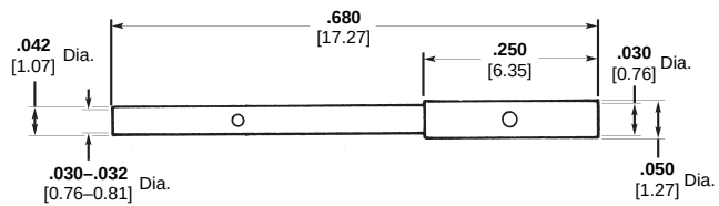
Part Number 096-0626-0001
