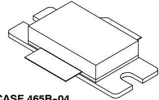
CASE 465B-04 NI-880 MRF7S21170HR3
