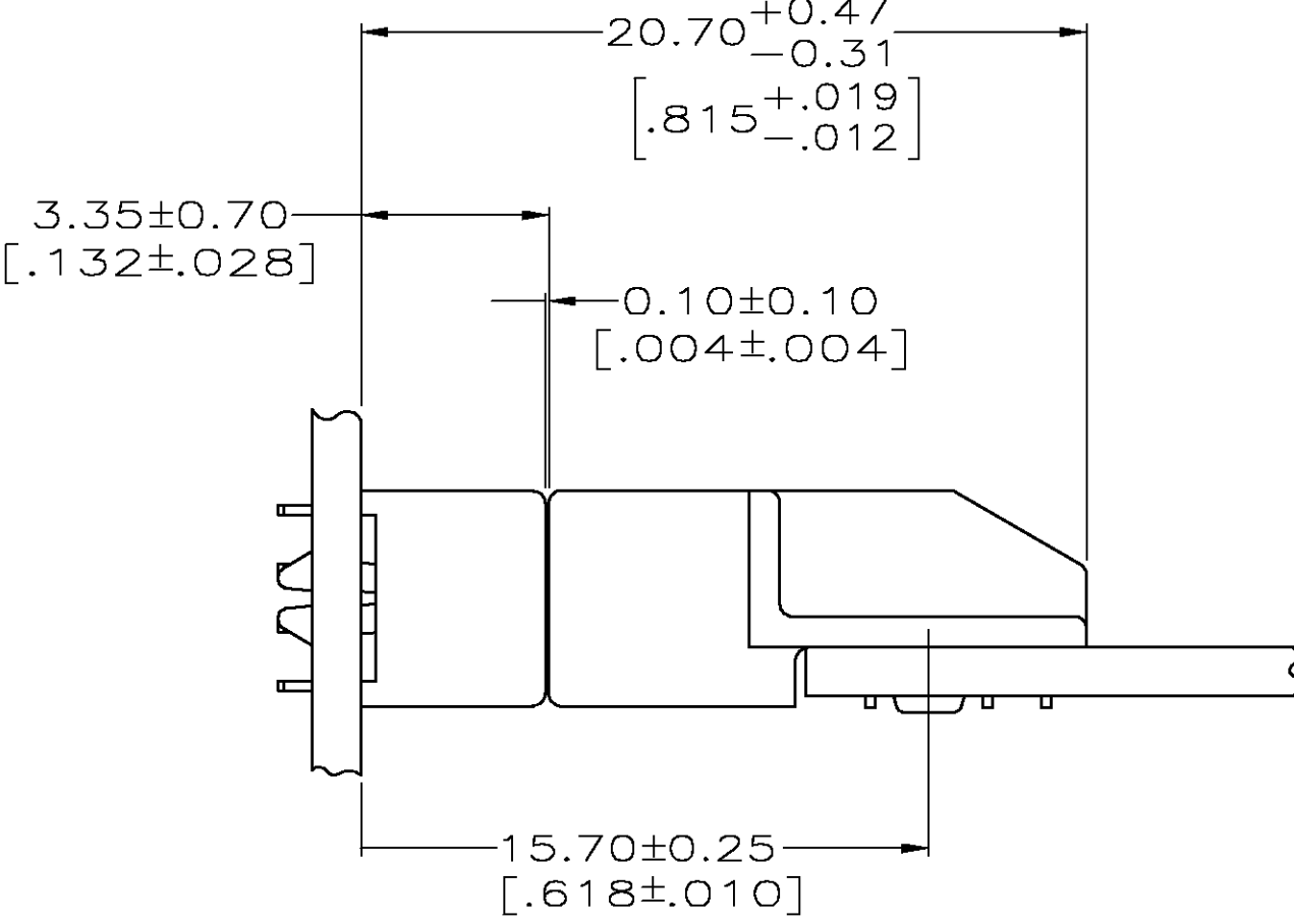
RIGHT ANGLE PLUG ASSEMBLY MATED TO VERTICAL RECEPTACLE ASSEMBLY
