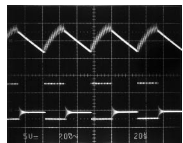
V OUTSW Burst Mode Operation at 1A Load
