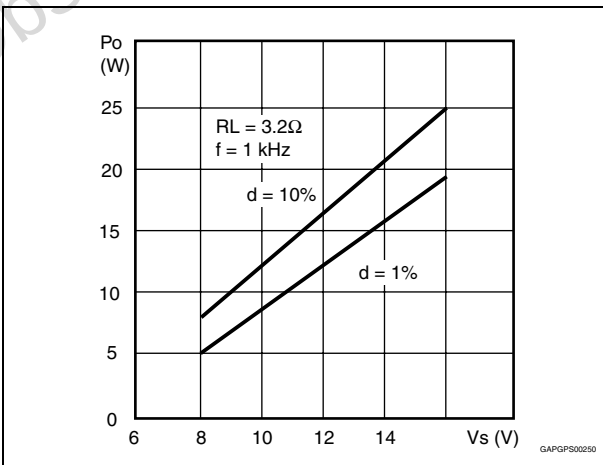
Figure 12. Output power vs. supply voltage (Bridge, 3.2 \Omega )
