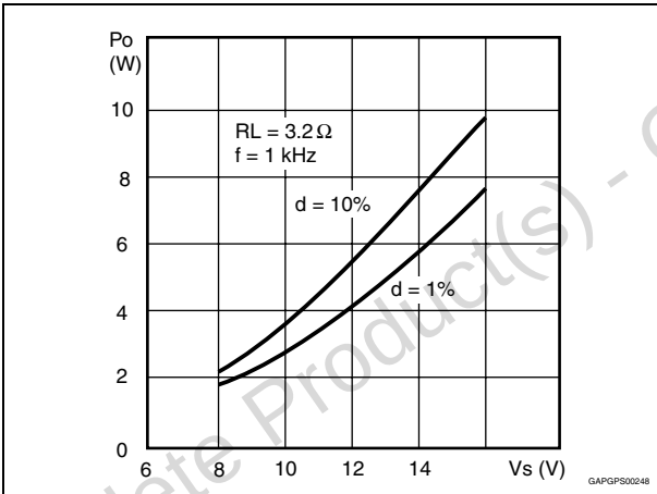
Figure 12. Output power vs. supply voltage (Bridge, 3.2 \Omega )
