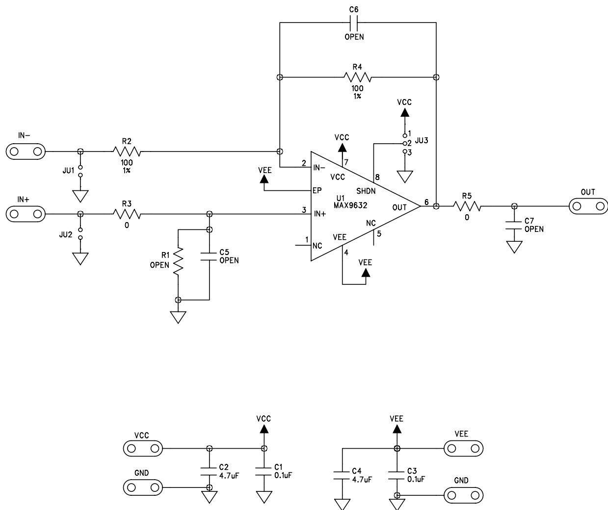
Figure 1. MAX9632 EV Kit Schematic
