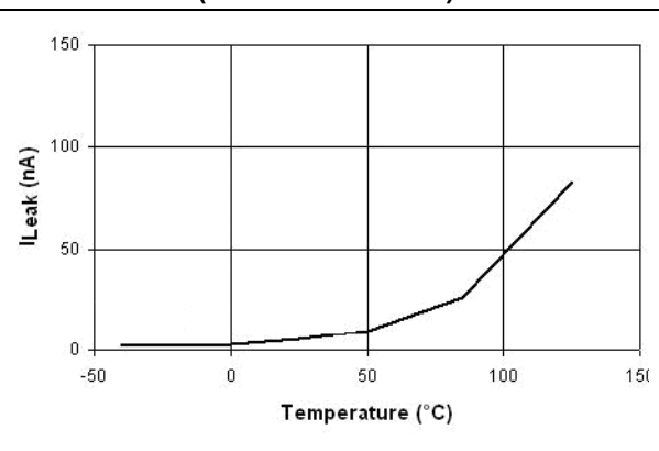
Figure 49. Switch leakage vs. temperature (STMP2161/2171)
