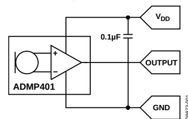
Figure 1. Evaluation Board Schematic
