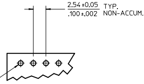
TYP. HOLE PATTERN FOR 1.57/.062 THK. PCB
