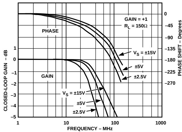
Figure 21. Closed-Loop Gain and Phase vs. Frequency, G = +1 , R_F = 1\text{ k}\Omega for \pm 15\text{ V} , 910\text{ }\Omega for \pm 5\text{ V} and \pm 2.5\text{ V}
