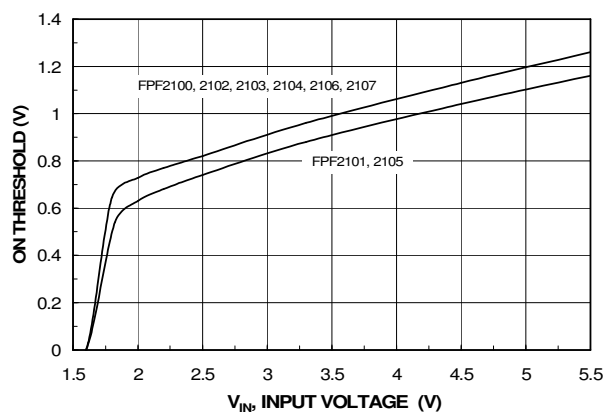
Figure 6. V_{IH} vs. V_{IN}
