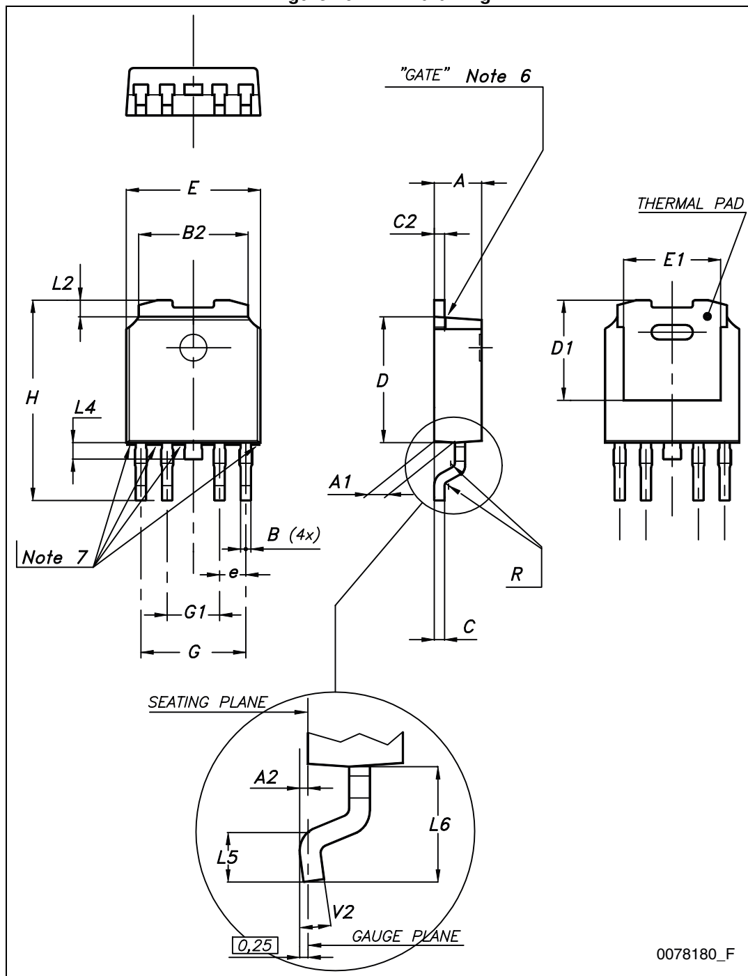
Figure 20. PPAK drawing
