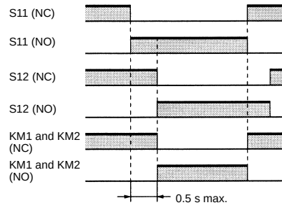
Timing Chart
