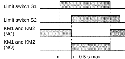
Timing Chart
