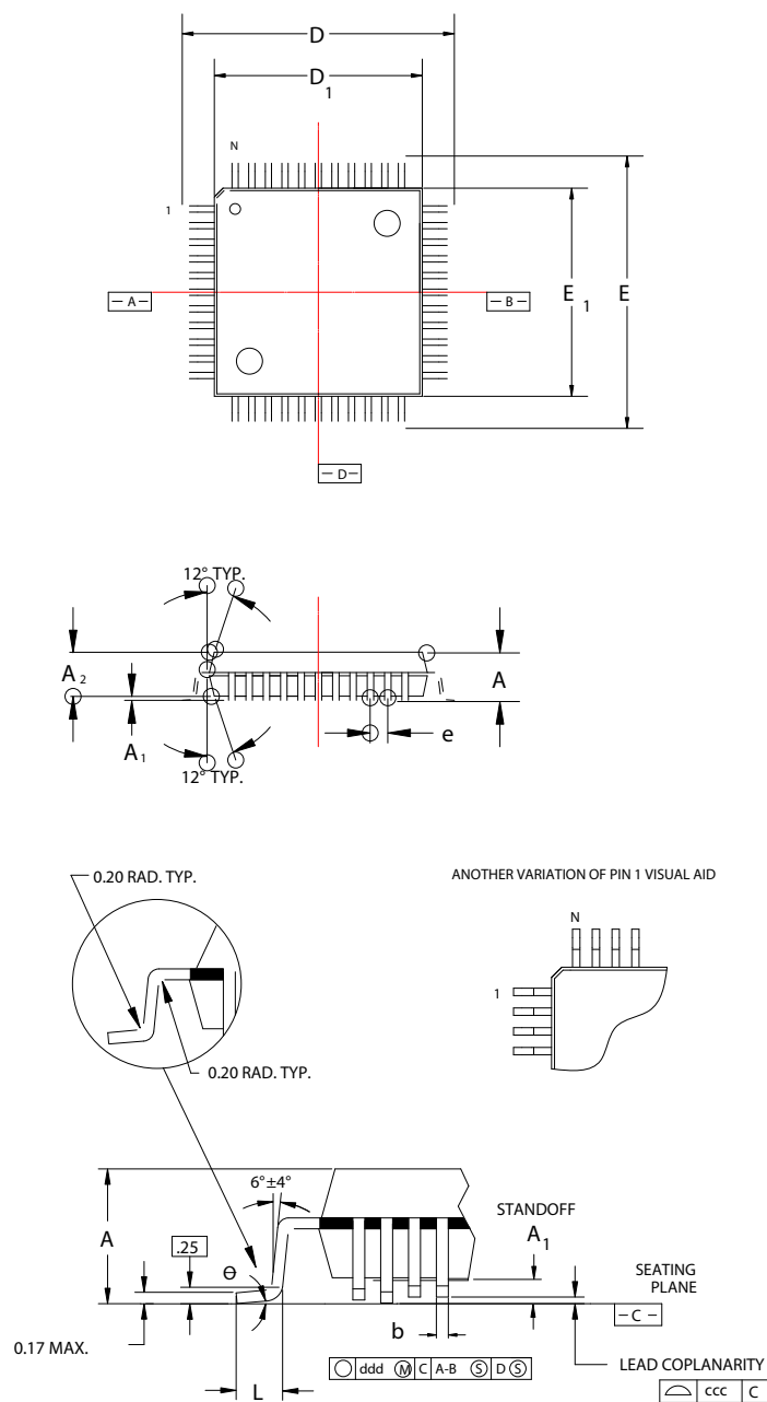
Figure C-1. Stellaris LM3S3N26 64-Pin LQFP Package
