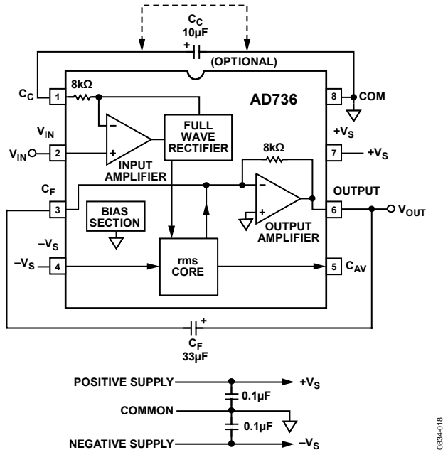
Figure 19. AD736 Average Responding Circuit
