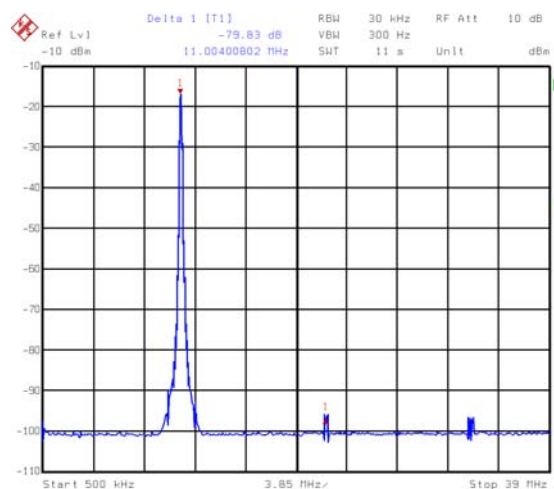
FIGURE 4. GSM AT 11MHz, 78MSPS CLOCK (79dBc - NYQUIST, 9dB PAD)
