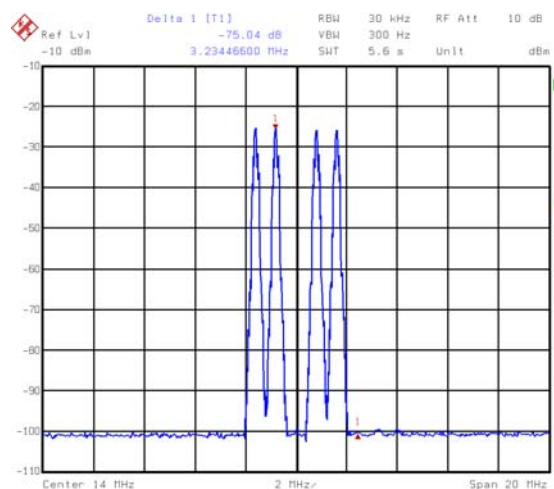
FIGURE 6. FOUR GSM CARRIERS AT 12.4-15.6MHz, 78MSPS (75+dBc - 20MHz WINDOW, 6dB PAD)
