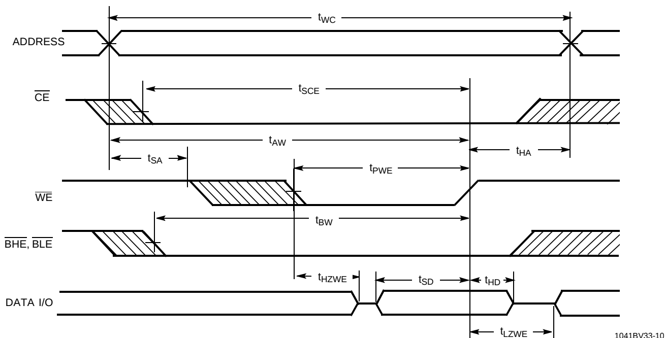
Write Cycle No.3 ( \overline{WE} Controlled, \overline{OE} LOW)
