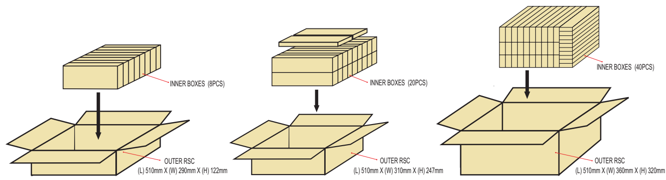
Figure 13. Dimensions for outer box packaging for LUXEON CoB (Gen 3).
