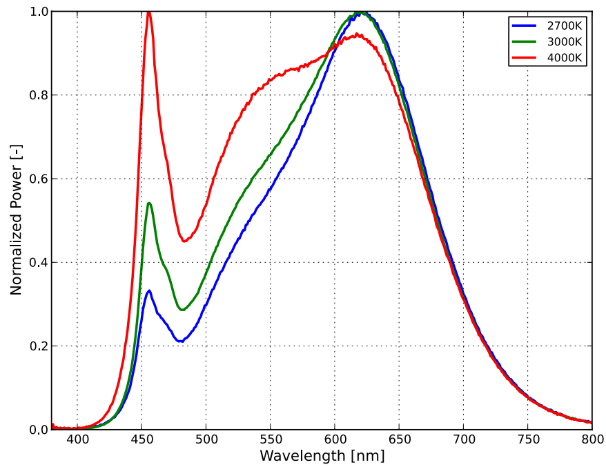
Figure 1c. Typical normalized power vs. wavelength for L2C5-xx9012xxxxx00 at specified test current, T_j=85^{\circ}\text{C} .
