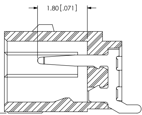
SECTION "A"-"A" SCALE 12 : 1
