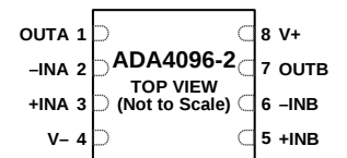
Figure 2. 8-Lead LFCSP (CP-8-10), ADA4096-2
