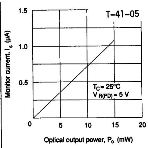
Figure 4 Optical Output Power vs. Monitor Current
