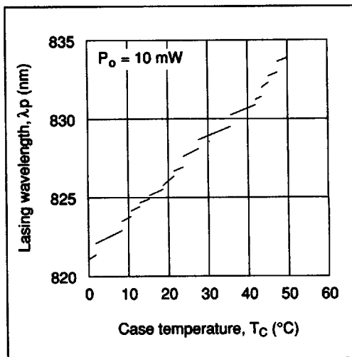
Figure 6 Temperature Dependence of Lasing Wavelength
