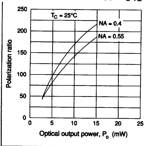
Figure 7 Optical Output Power Dependence of Polarization Ratio
