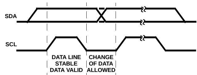
FIGURE 16. DATA VALIDITY
