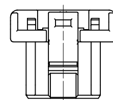
4,5極形状 (1ロック) FIGURE OF 4,5 CIRCUIT (1 LOCK)
