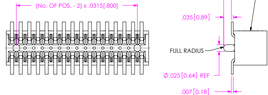
FIG 4 -A OPTION (MOLDED) 4 POSITIONS MIN
