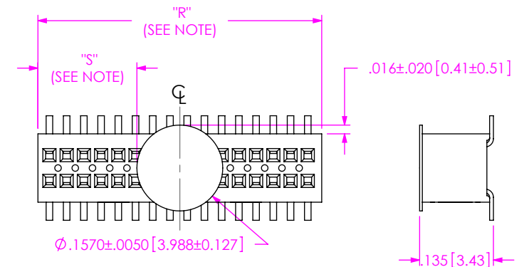
FIG 5 -K: POLYIMIDE FILM PAD 8 POSITIONS MIN
