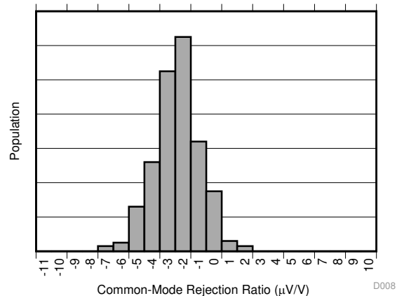
Figure 8. Common-Mode Rejection Production Distribution (INA381A3)
