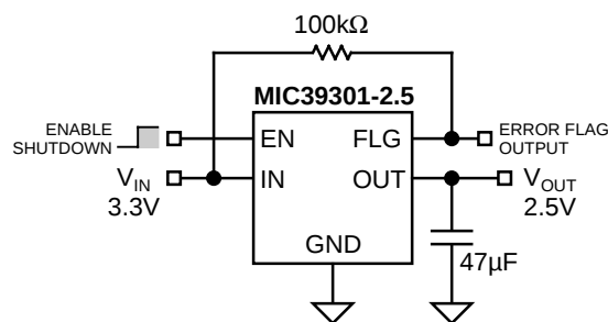
MIC39301
