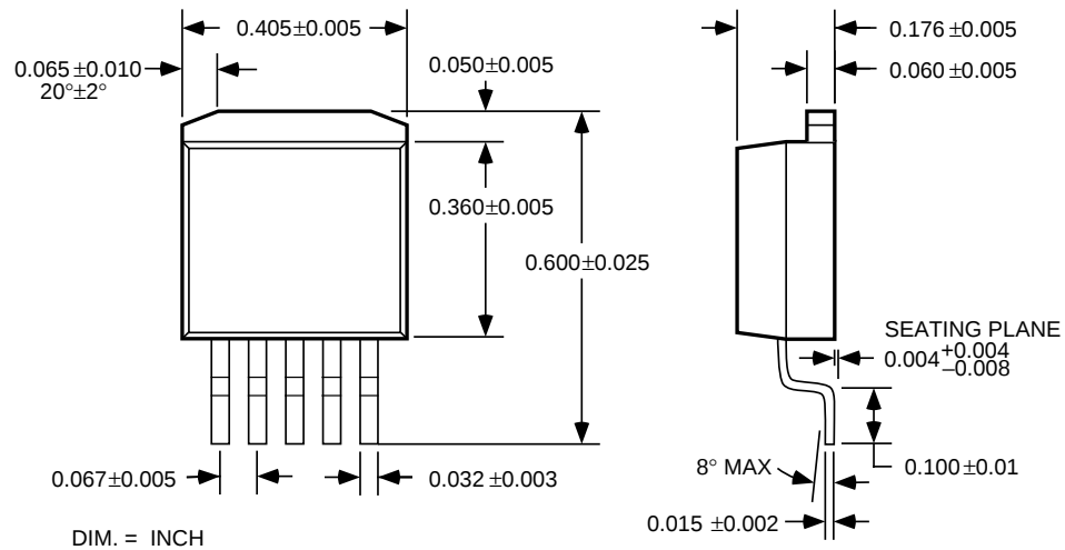
5-Lead TO-263-5 (U)
