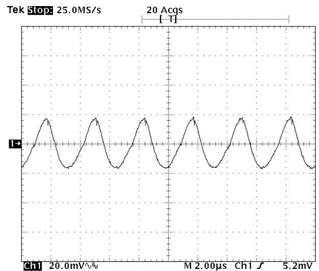
Fig-1.0V-5: Output voltage ripple (20mV/div.) for Vout=1.0V at full rated load current into a resistive load with external capacitance 47 \mu Fx4 ceramic + 1 \mu F ceramic at Vin=5.0V.
