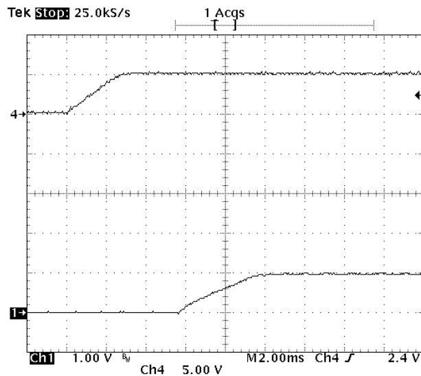
Fig-1.0V-4: Turn-on transient for Vout=1.0V with application of Vin at full rated load current (resistive) and 47 \mu Fx4 external capacitance at Vin=5.0V.
