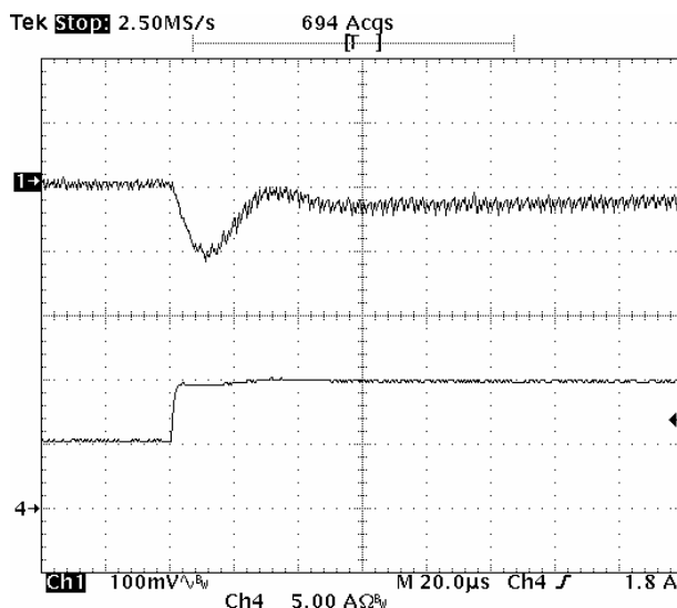
Fig-1.0V-6: Output voltage response for Vout=1.0V to positive load current step-change from 5A to 10A with slew rate of 5A/ \mu s at Vin=5.0V. Co=47 \mu Fx4 ceramic +1 \mu F ceramic.
