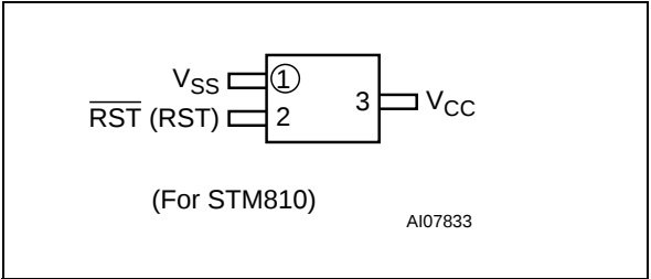
Figure 4. SOT23-3 Connections
