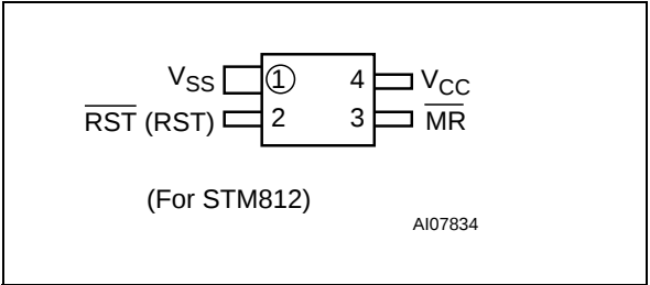
Figure 5. SOT143-4 Connections
