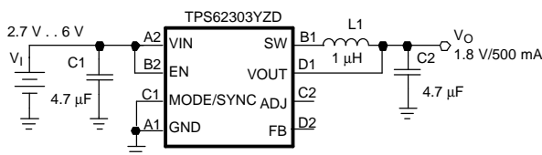
Figure 1. Smallest Solution Size Application (Fixed Output Voltage)
