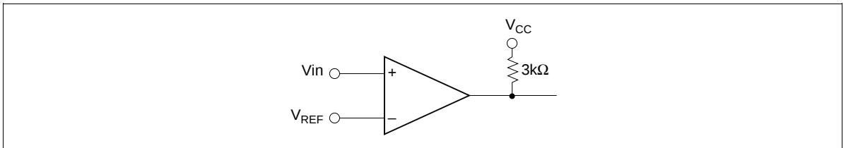
Figure 6 Basic Comparator
