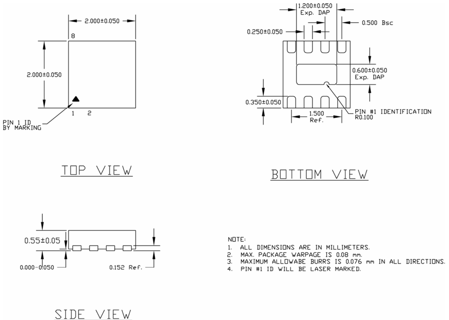
8-Pin 2mm x 2mm Thin MLF ® (MT)
