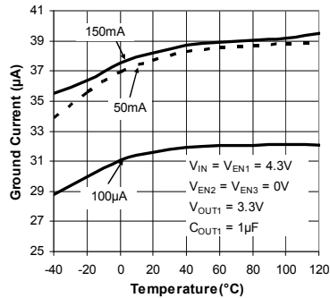
Ground Current vs Temperature (single output)
