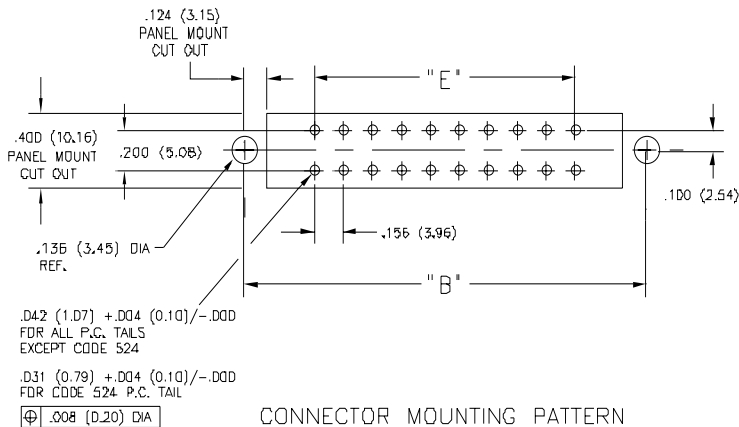
CONNECTOR MOUNTING PATTERN
