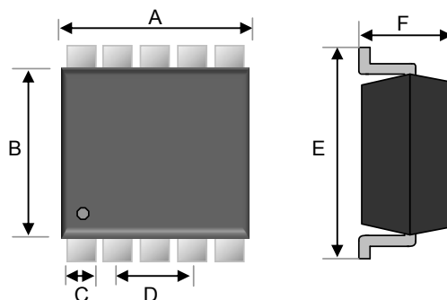
MSOP-10
