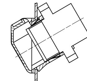
VERSION 4 (MTP-MTP) SEE NOTE 2
