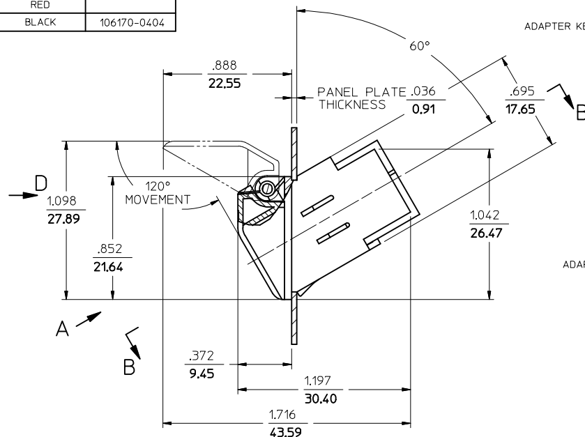
VERSION 2 (FC-SC) DOOR REMOVED ROTATED 30° CW
