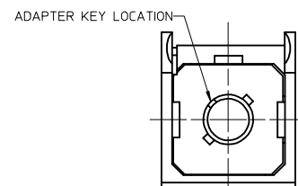
VERSION 1 (ST-SC) DOOR REMOVED ROTATED 30° CW
