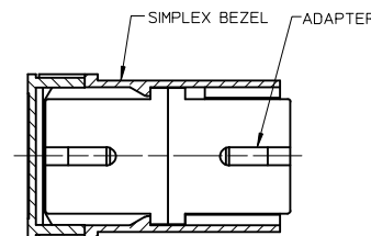
VERSION 3 (SC-SC) ROTATED 30° CW
