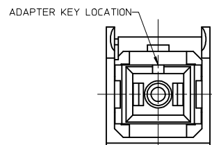
VERSION 3 (SC-SC) DOOR REMOVED ROTATED 30° CW
