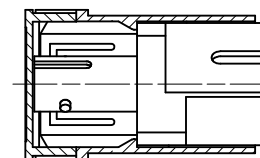
VERSION 1 (ST-SC) ROTATED 30° CW
