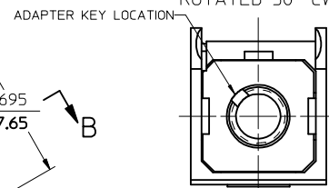
VERSION 2 (FC-SC) DOOR REMOVED ROTATED 30° CW
