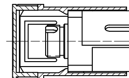
VERSION 2 (FC-SC) ROTATED 30° CW
