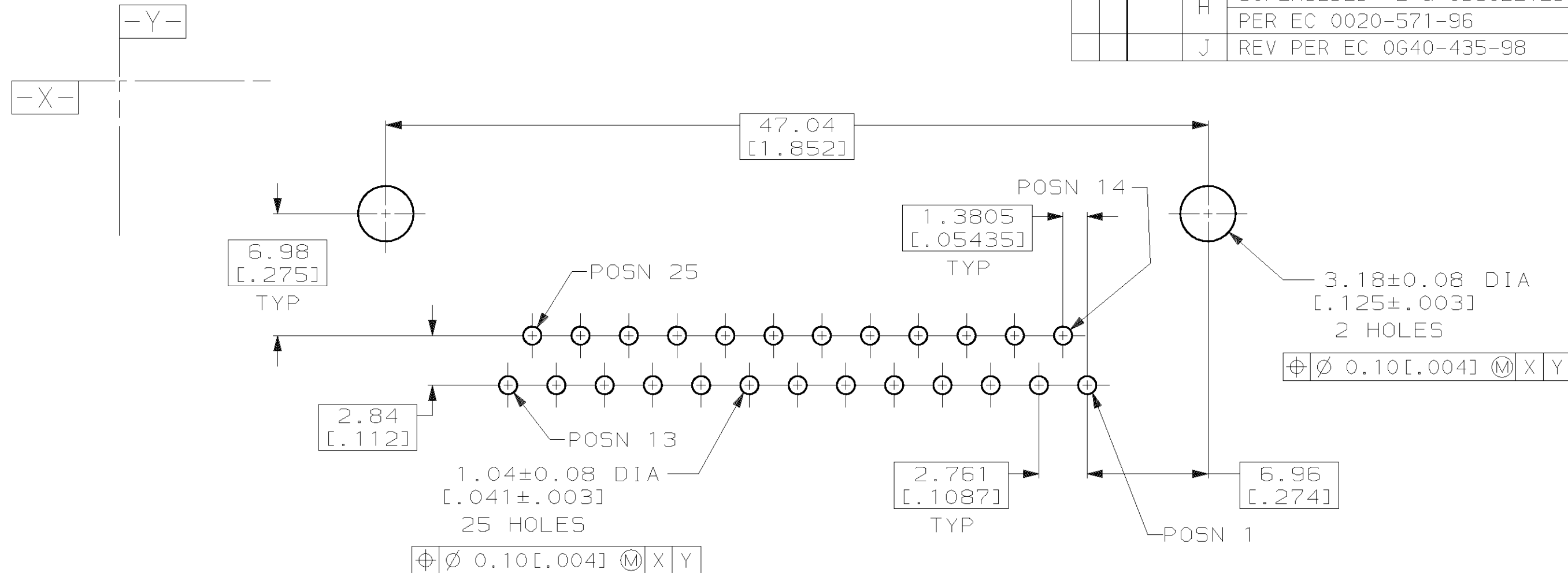
5.99 [.236] -B- 18.92±0.38 [.745±.015] 1.27 [.050] 10.03±0.25 [.395±.010] 3.18±0.51 [.125±.020] TYP 0.213±0.010 [.0084±.0004] 25 PLC ⊕ 0.38 [0.015] Ⓜ C A Ⓢ B
