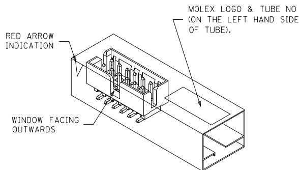
FIG.1 : ORIENTATION OF PART IN TUBE.
