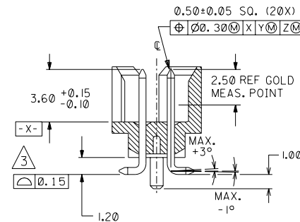
SECTION G-G
