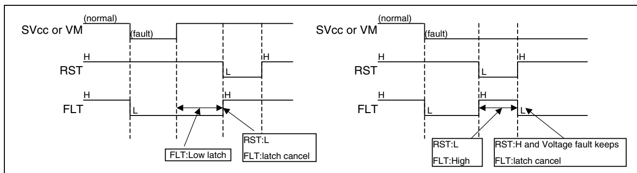
Fig.10 Voltage Monitor Circuit &amp; Timing Chart
