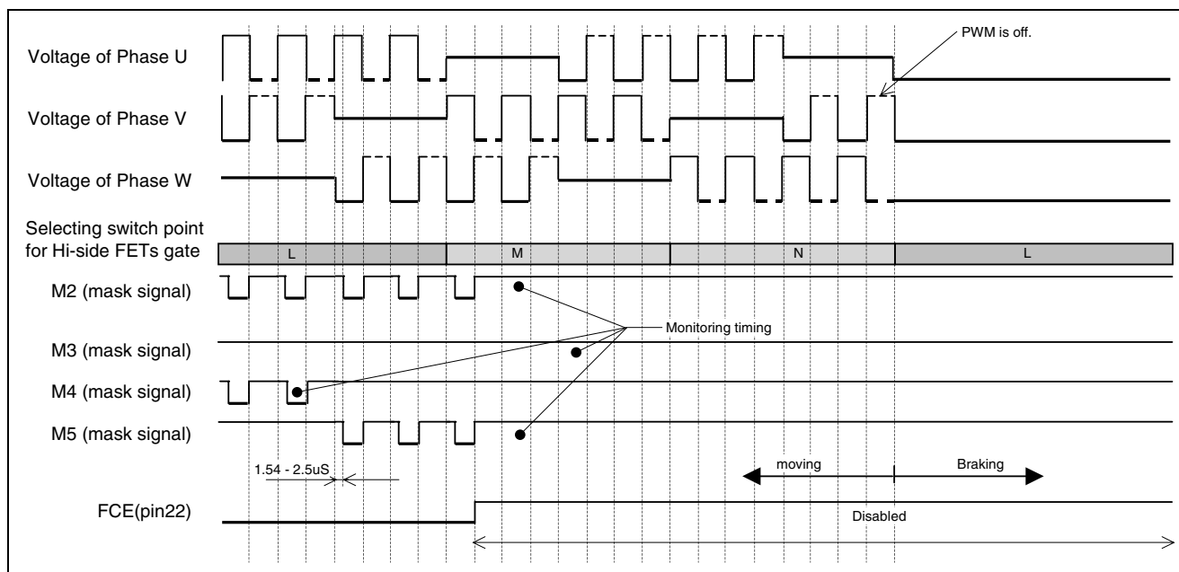
Fig.22 Timing chart of gate voltage monitor in Fast Decay
