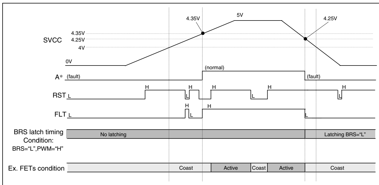
Fig.24 Timing chart in power on and off (Pattern A)
