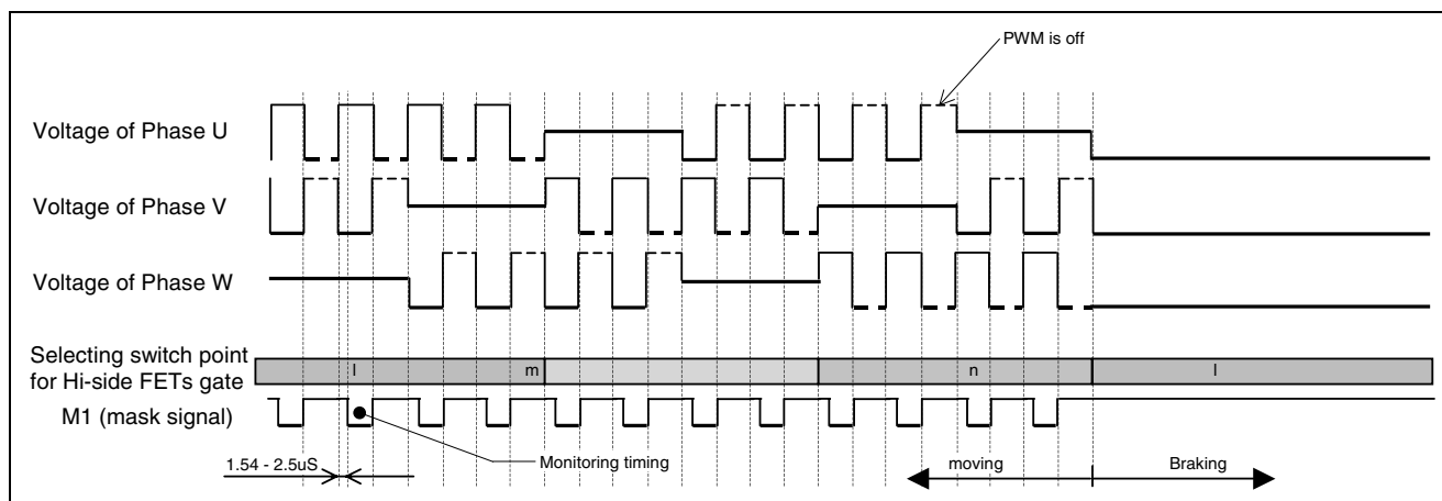
Fig.21 Timing of drain-source voltage monitor
