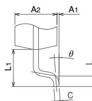
Detail F
