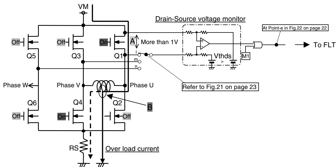
Fig.20 Drain-Source voltage monitor of external FETs
