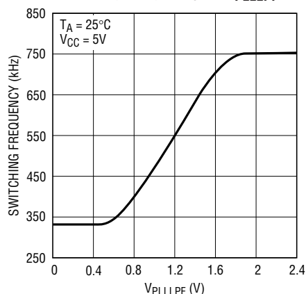
Switching Frequency vs V_{PLL\text{PF}}
