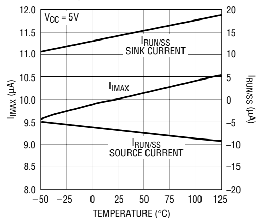
I_{\text{MAX}} and I_{\text{RUN/SS}} vs Temperature
