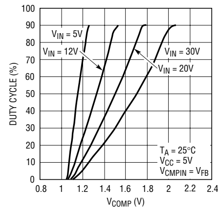
Duty Cycle vs V_{C\text{COMP}}
