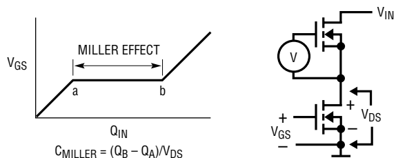
Figure 8b. Gate Charge Characteristics
