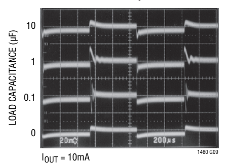
2.5V Transient Responses
