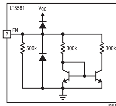
Figure 14. Enable Pin Simplified Schematic
